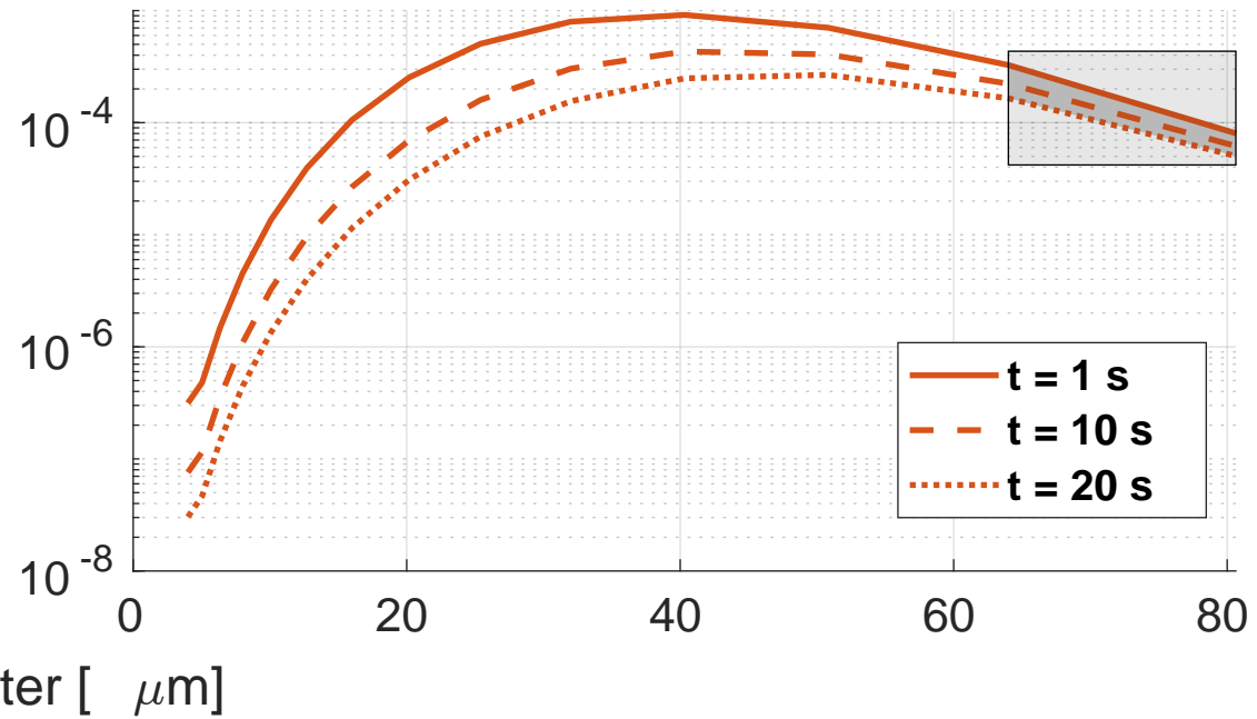
(b) bin-SBM
