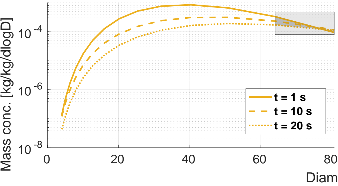
(a) AMP-SBM
