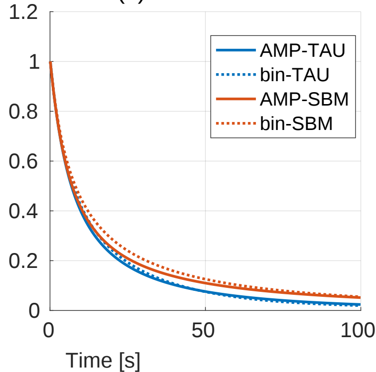
(b) Cloud mass
