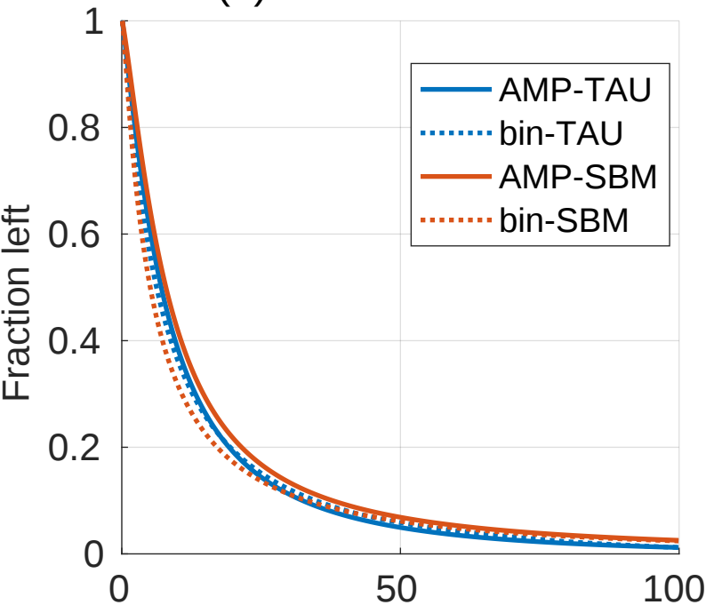
(a) Cloud number
