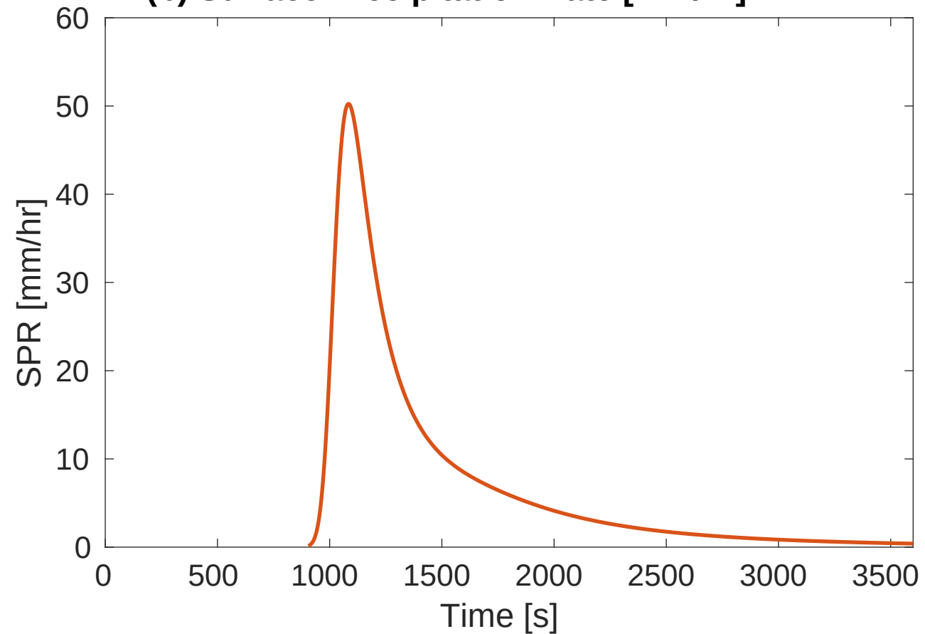
(b) Surface Precipitation Rate [mm/hr]
