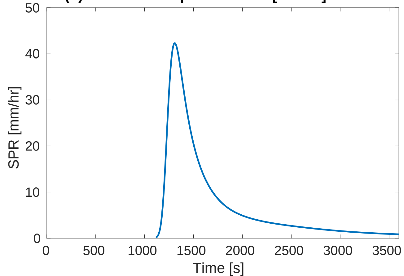
(b) Surface Precipitation Rate [mm/hr]
