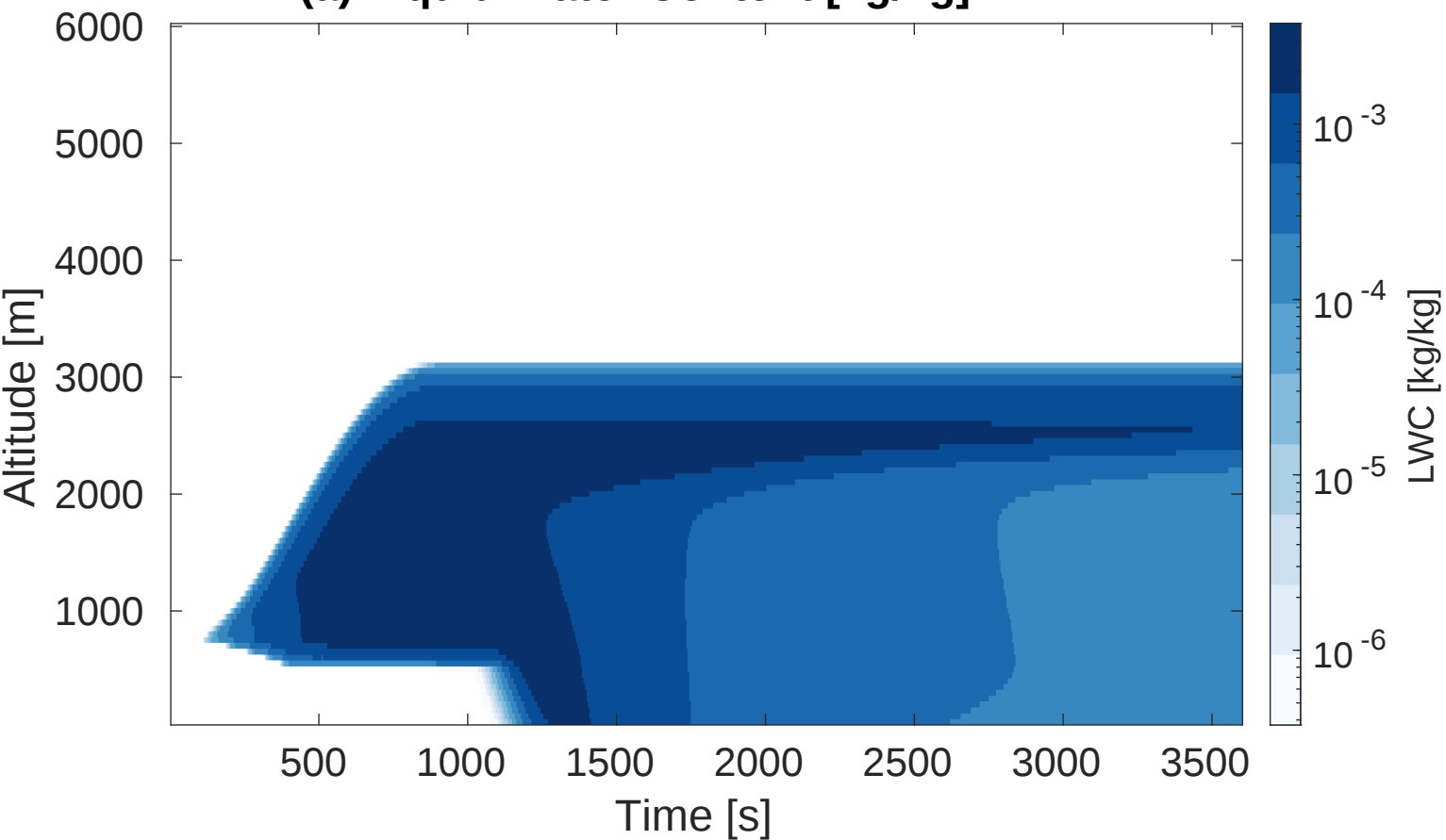
(a) Liquid Water Content [kg/kg]
