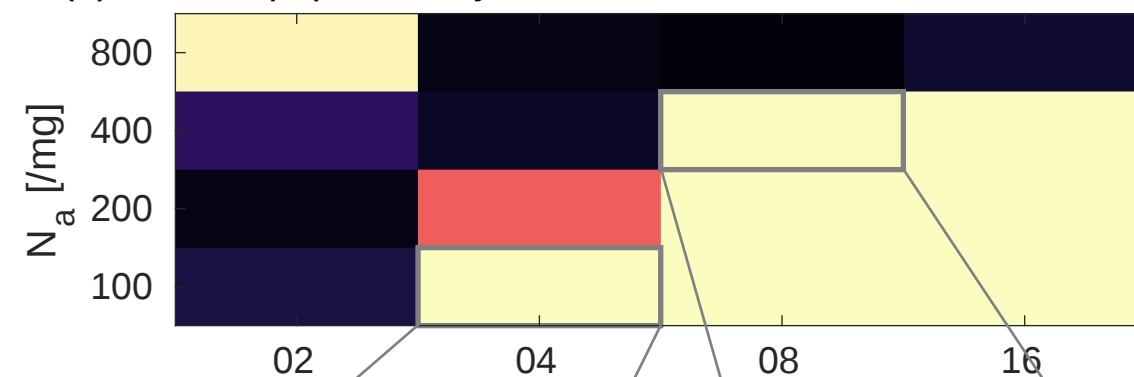
(b) surface pcpt. rate by S-AMP-TAU, mean score = -0.553
