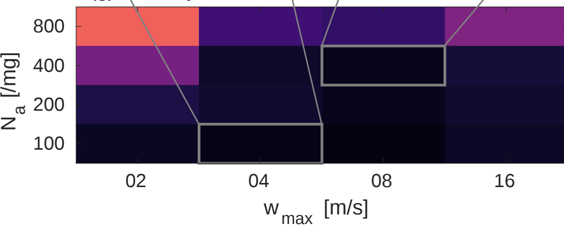
(g) CWP by U-AMP-TAU, mean score = 0.815
