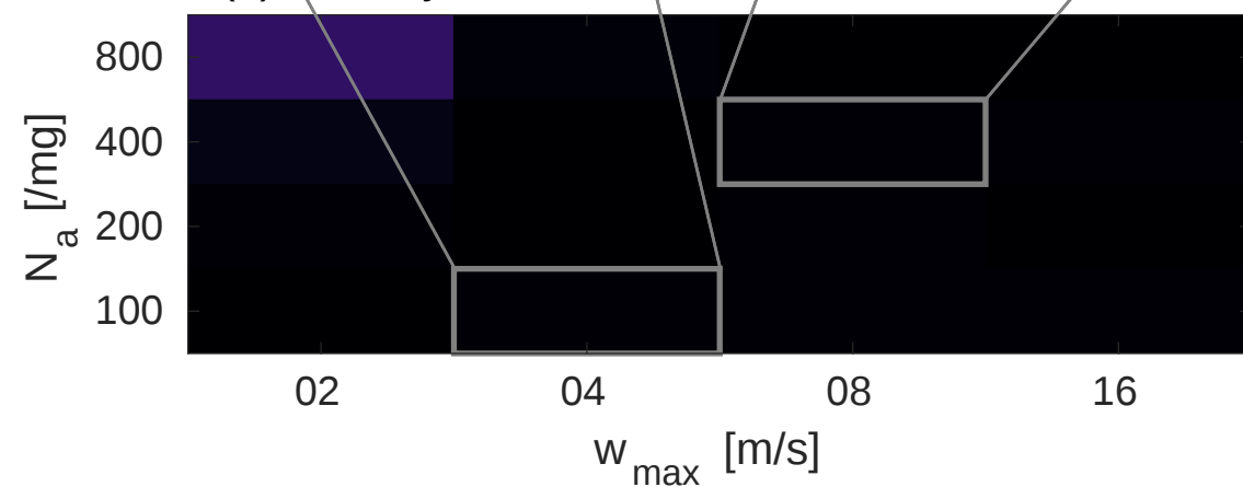
(h) LWP by U-AMP-TAU, mean score = 0.987
